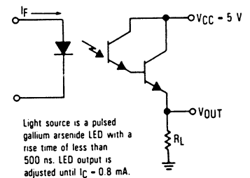
Switching Time Test Circuit
